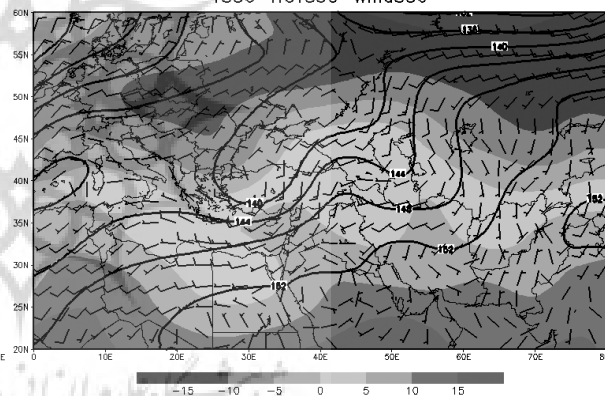
T850-HGT850-Wind850
