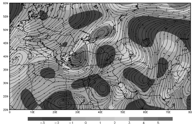
VOR850-Stream850
