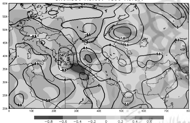
SHUM850 Advect-T850 Advect
