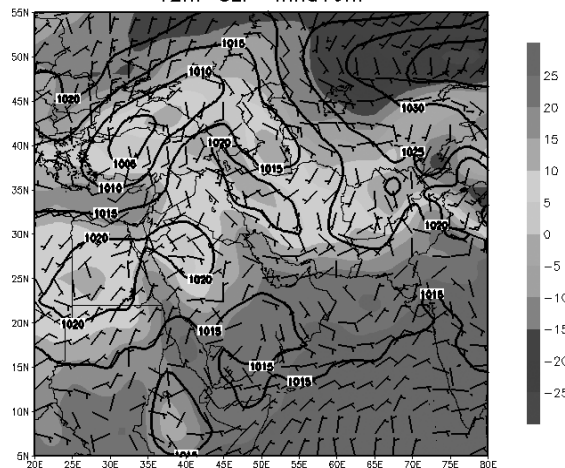
T2m-SLP-Wind10m
