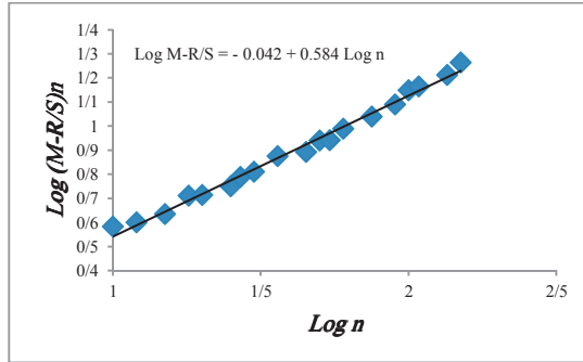
Figure 4(b): Estimation of the Hurst exponent based on the M-R/S technique for the period: 2002:21:03-2010:17:06
