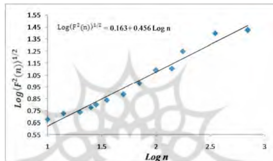
Figure 3(c): Estimation of the Hurst exponent based on the DFA technique for the period: 1999:25:01-2002:21:03
