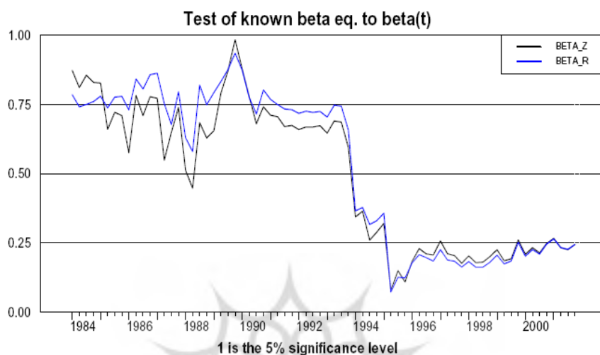
Figure 1: Recursive Likelihood Ratio Tests for Interest-Free Monetary Aggregate
