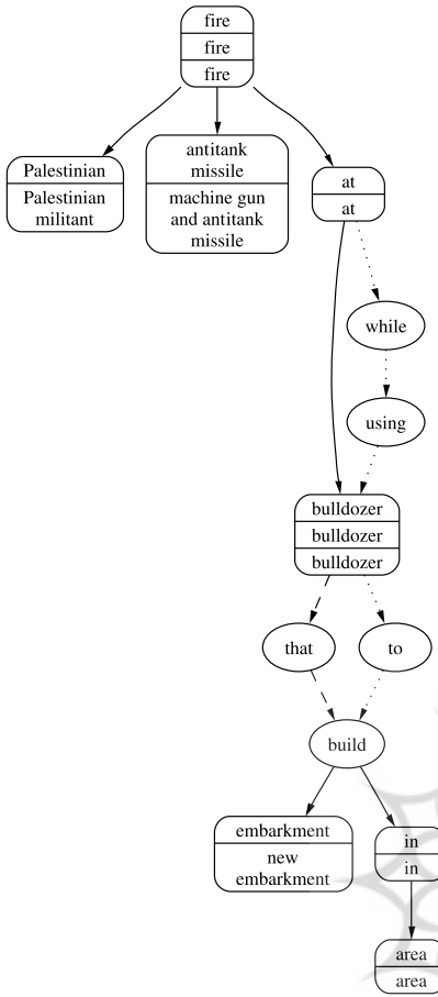
Figure 7 A pruned basis lattice.
