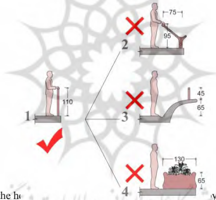
Figure 5. Reductionist view in setting the height of the railing by the building regulations.
