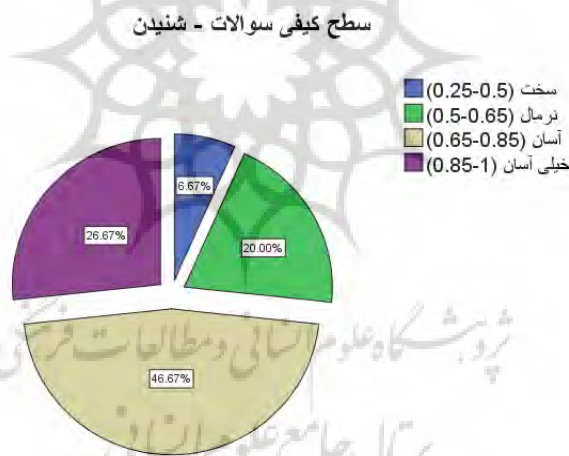
Graph 1. Frequency Distribution of Difficulty Coefficient of Listening Comprehension Questions
