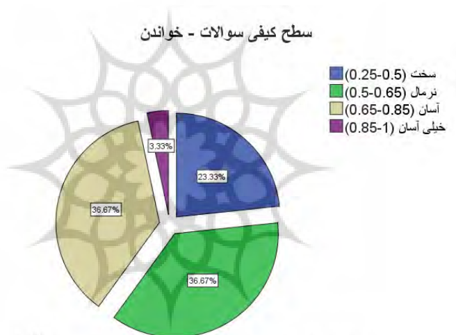
Graph 2. Frequency Distribution of Difficulty Coefficient of Reading Questions
