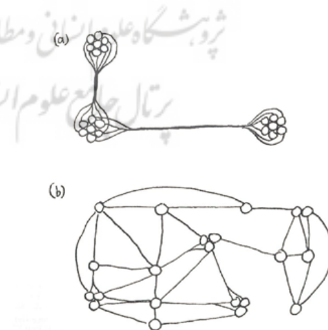
▲ Diag 5. Connecting nodes of human activity; Connective paths are multiple and irregular: a) Nodes are concentrated into three clusters with all connections forced into two channels; b) The same nodes distributed with connections that work much better (city and urban blocks)(Salingaros, 2005 & 2008)
