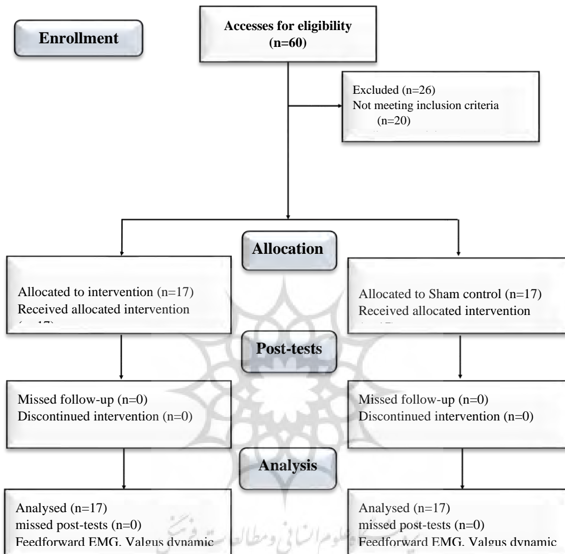
Fig 1. Study flowchart.
