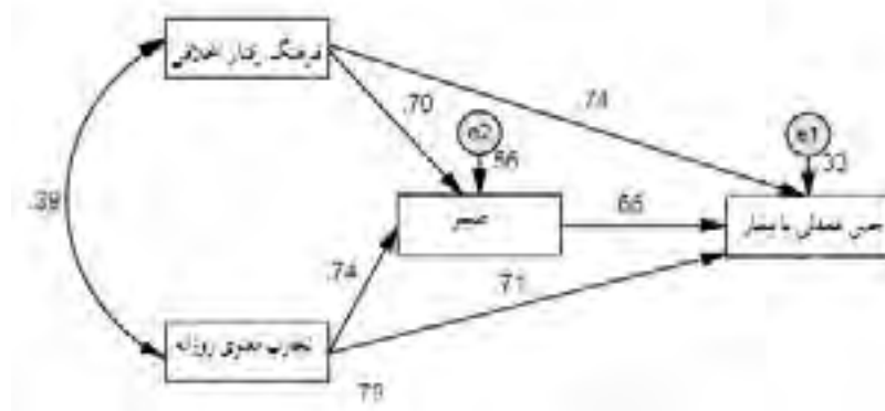
Figure 1. The final model of the research along with the standard coefficients of the paths
