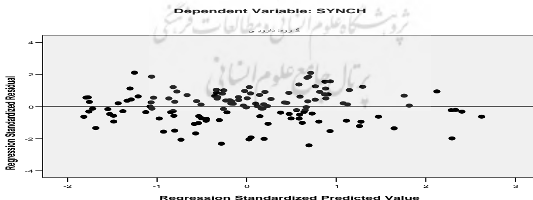
Scatterplot
