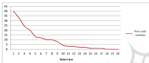
Diagram 1. Theoretical saturation process
