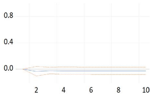
Response of GINI to LPOLR
