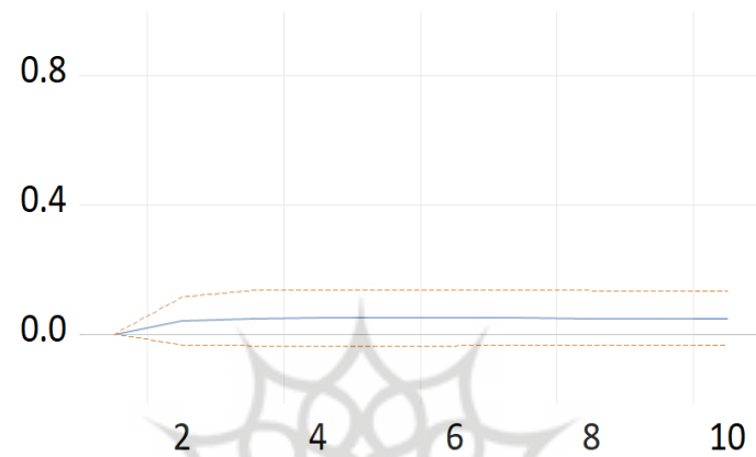
Response of GINI to GINI
