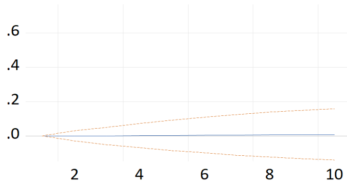
Response of GINI to LLFINR
