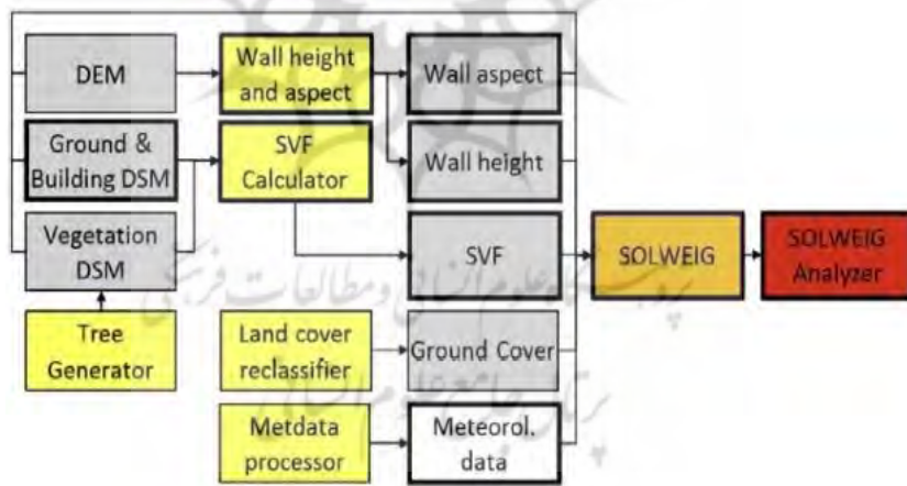
Fig.8. Structure of modules and calculation analysis in SOLWEIG (Lindberg et al., 2018)
