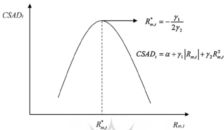
Figure 1. The nonlinear relationship between CSAD_t and R_{m,t}
