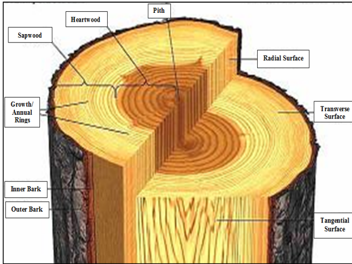
Fig. 2. The Anatomy of a Tree Trunk (Parsa Pajouh and Schweingruber, 1988)
