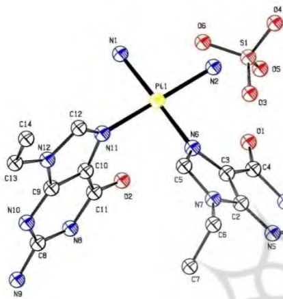
cis -[Pt(NH 3 ) 2 (9-Ethylguanine)](SO 4 )
