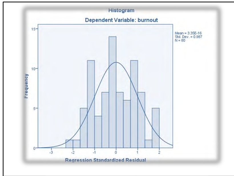
Figure 1. Histogram
