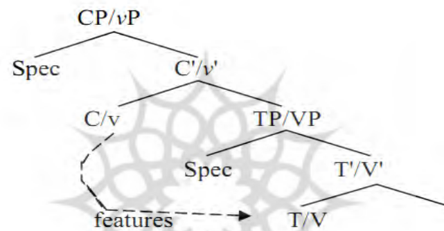
Chart 3. Feature Inheritance
