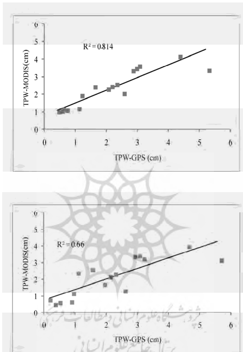
Fig 8. Comparison between TPWs Extracted from GPS with those Retrieved from MODIS Algorithm (Lower) and those Modified with our Technique (Upper).
