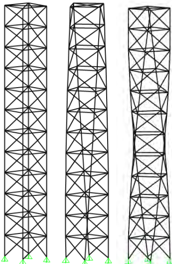
Fig. 16 form of columns with 0, 45, and 90 degrees (The rotation states of 22.5, 67.5 and 135 degrees have not been displayed)
