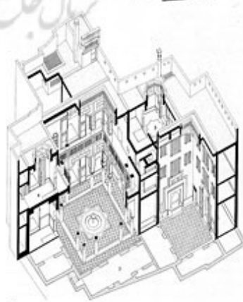
۵۳ Axonometric section, ground floor and first floor plans of a double courtyard house in Fez, serving a large family and embracing several semi-independent sub-units. The house is located in a privileged position between three residential clusters, allowing the owners to accede from different dead-end alleys. 1. Main entry 2. Side entries from other lanes 3. Typical living unit (bait) 4. First floor apartment composed of two small baits and its own central light shaft 5. Separate upper-floor apartment (marzaj)
