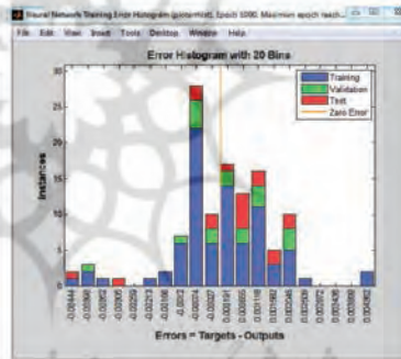
error histogram
