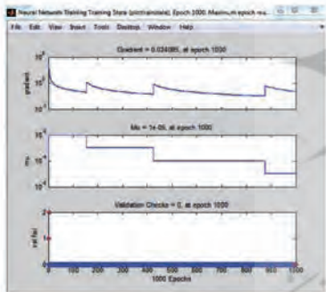
training state
