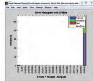
error histogram
