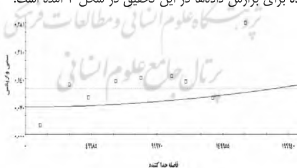
Gaussian model (Co=0.0530, Co+C=0.3296, A1=924000.00, A2=319000.00; r2=0.208; RSS=0.170)
