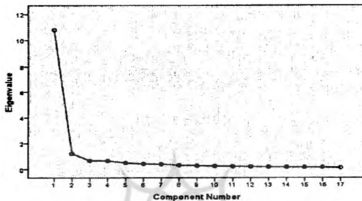
Scree Plot
