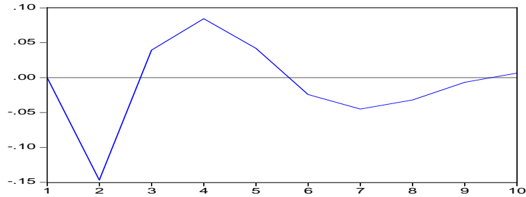
Response of LTBW to Cholesky One S.D. LRERW Innovation
